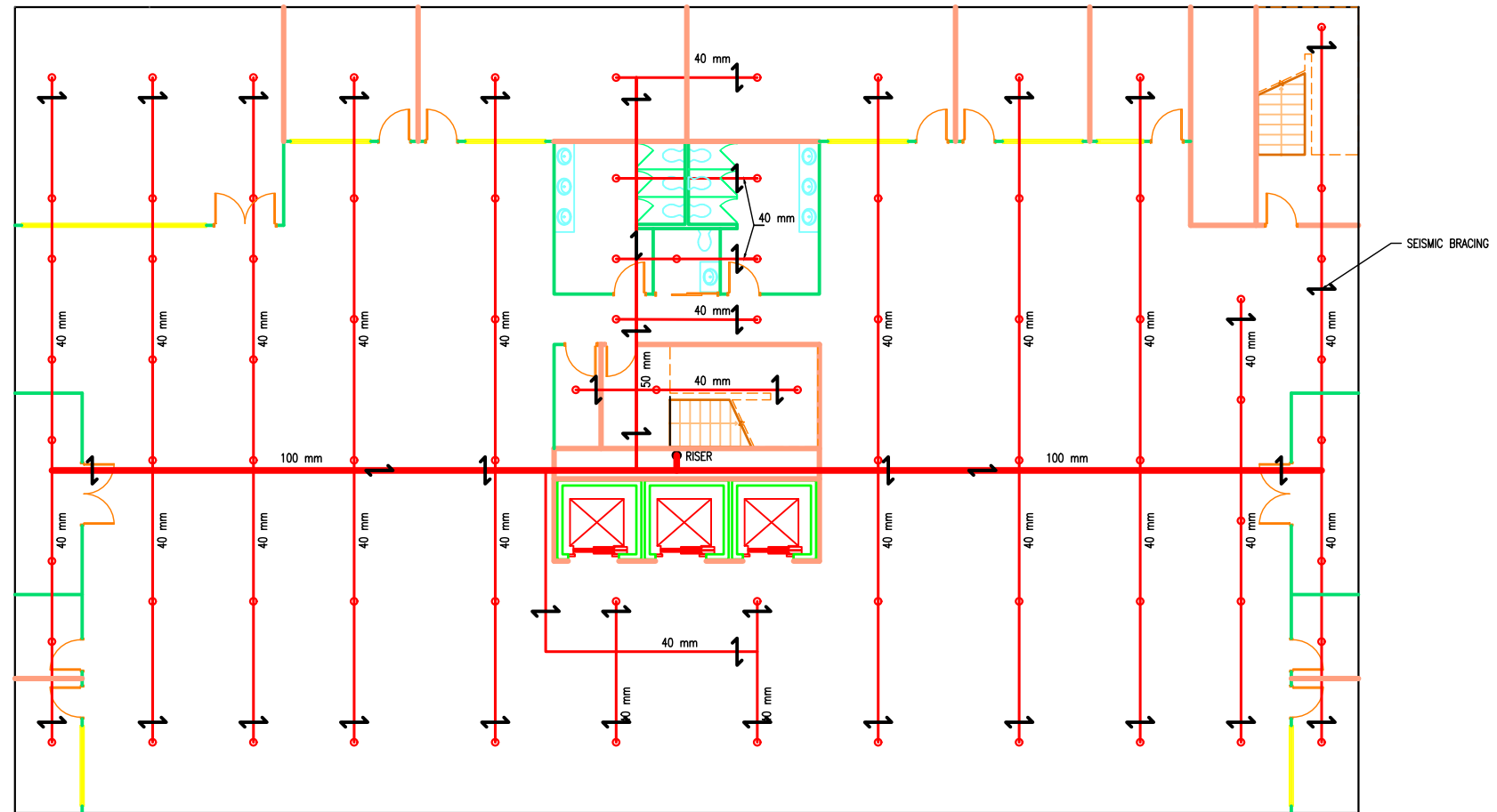
SPRINKLER LAYOUT FOR UPPER FLOORS (SCALE 1:200, UNITS IN MM)
