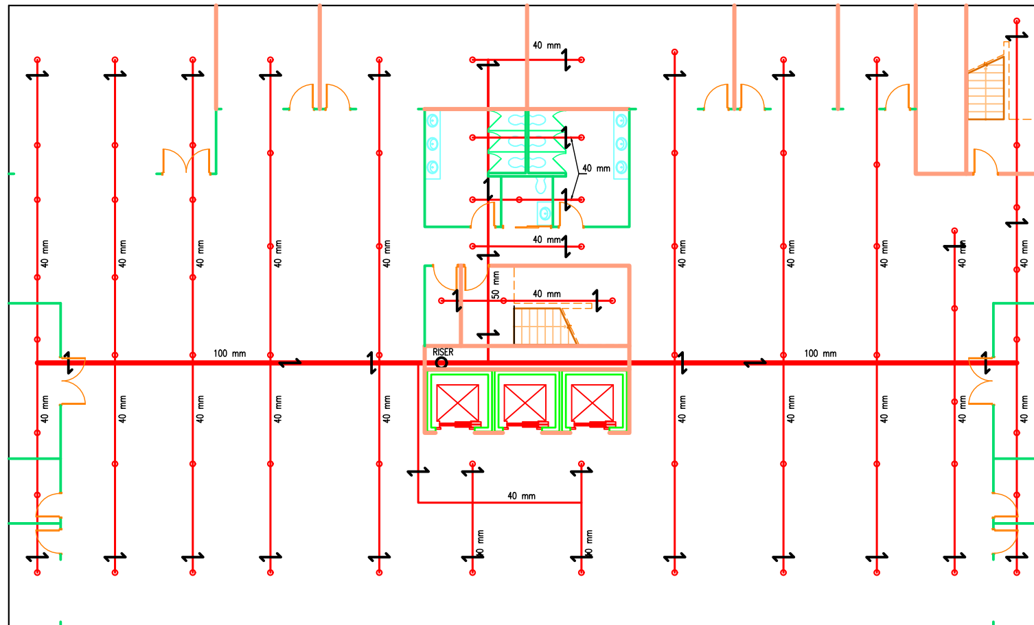
SPRINKLER LAYOUT FOR UPPER FLOORS (SCALE 1:200, UNITS IN MM)
