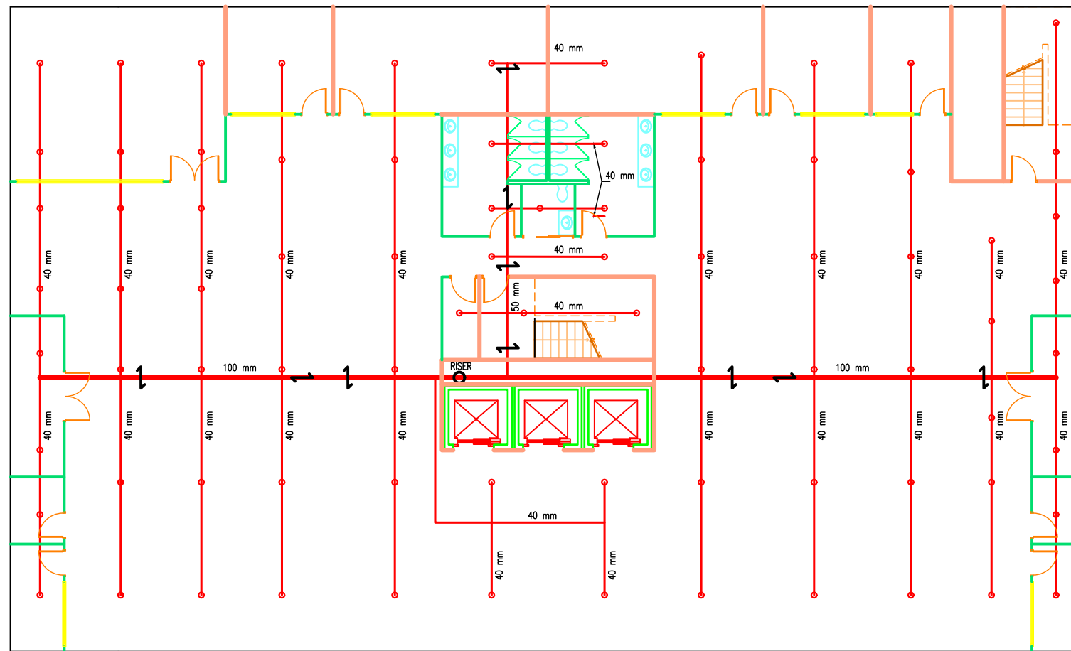
ABOVE CEILING LAYOUT FOR UPPER FLOORS (SCALE 1:200, UNITS IN MM)
