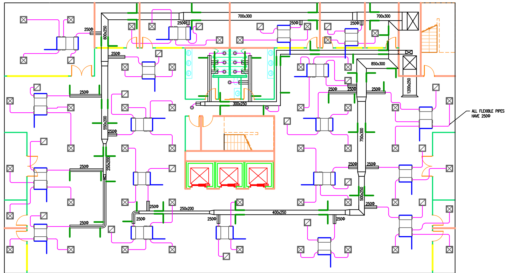
HVAC LAYOUT FOR UPPER FLOORS (SCALE 1:200, UNITS IN MM)
