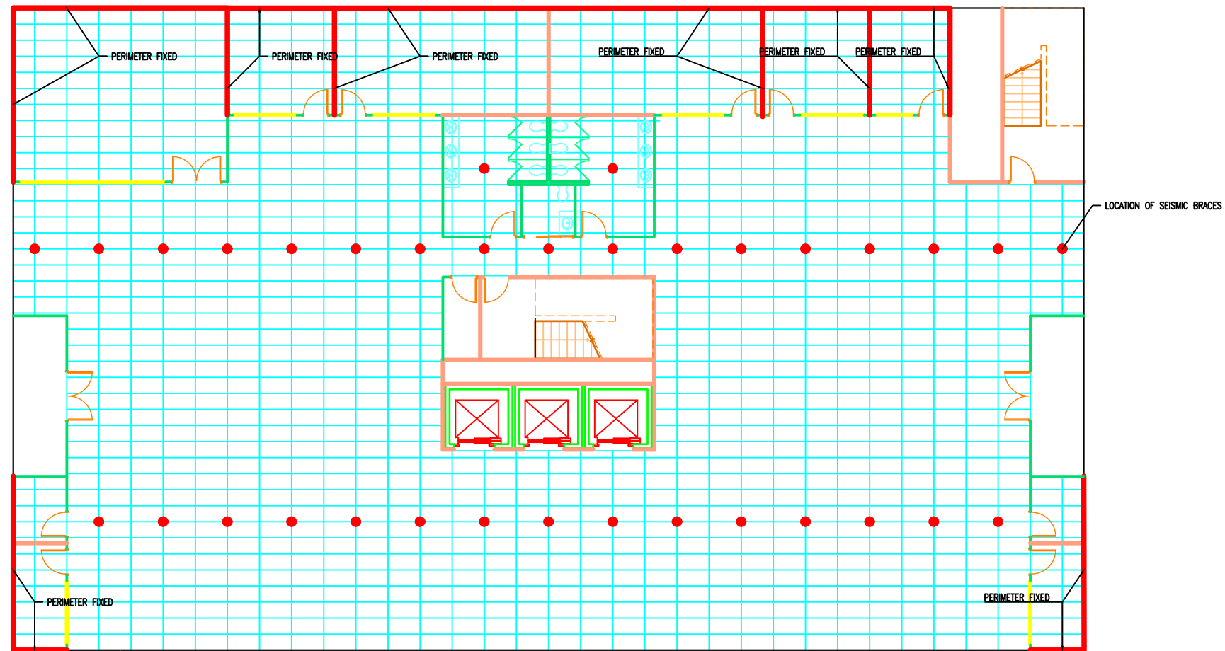
CEILING LAYOUT FOR UPPER FLOORS (SCALE 1:200, UNITS IN MM)
