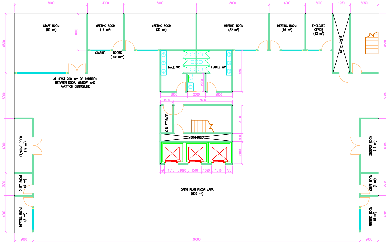
UPPER FLOOR LAYOUT (SCALE 1:200, UNITS IN MM)
