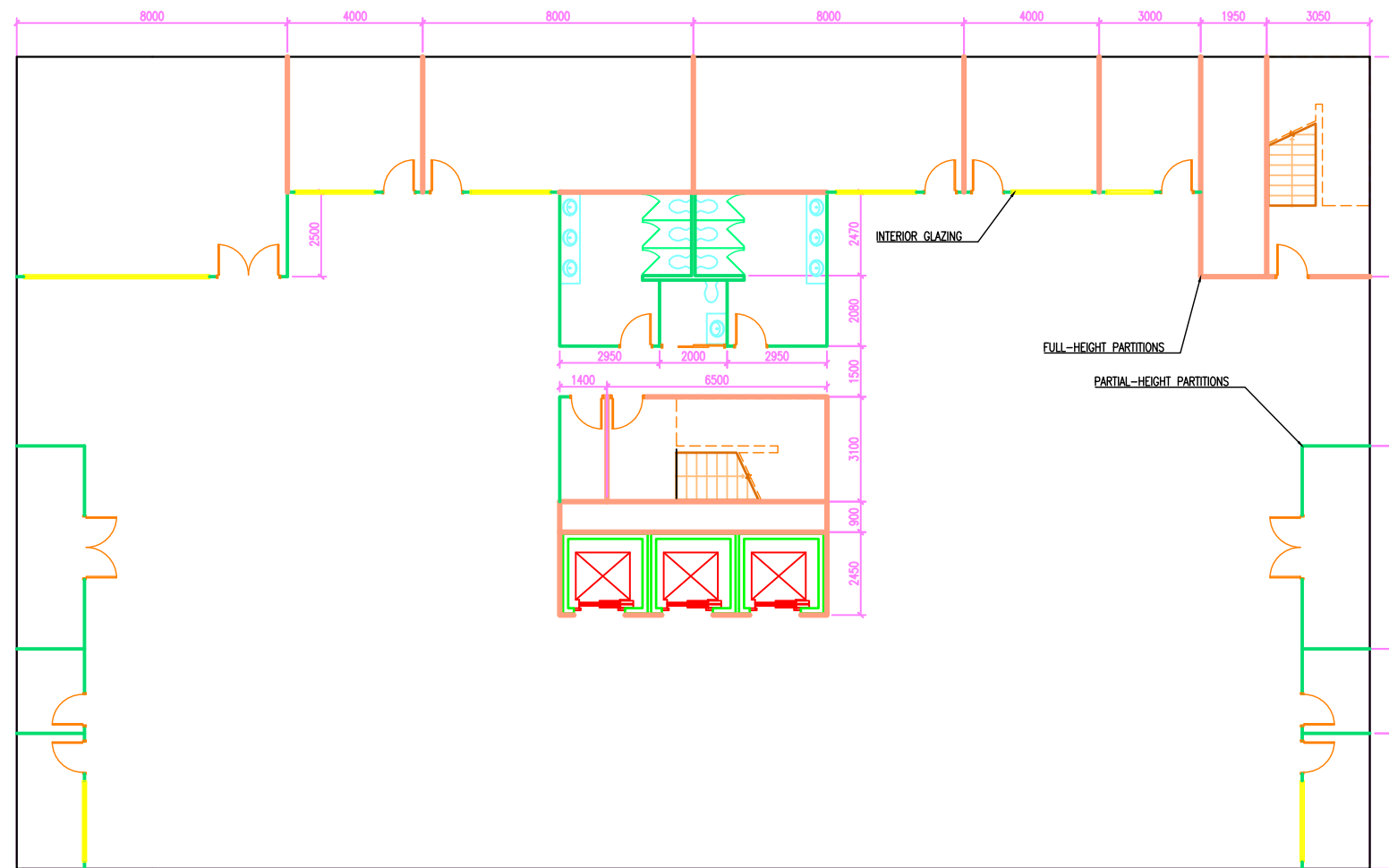
ROOM AND PARTITION LAYOUT FOR UPPER FLOORS (SCALE 1:200, UNITS IN MM)
