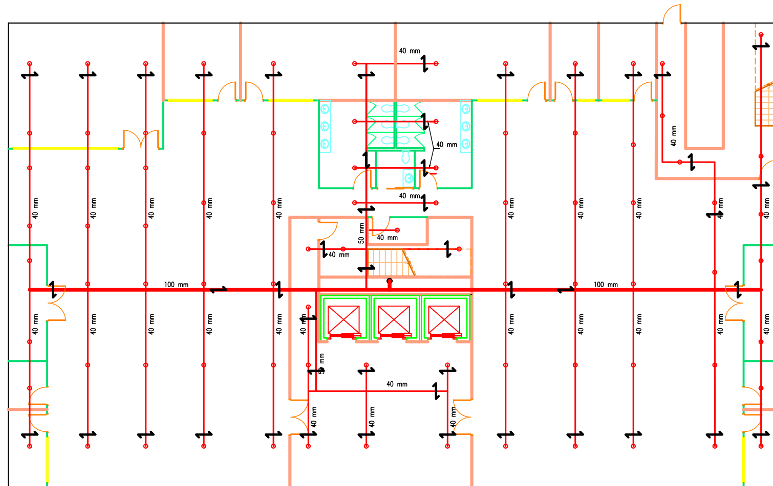
SPRINKLER LAYOUT FOR GROUND FLOOR (SCALE 1:200, UNITS IN MM)
