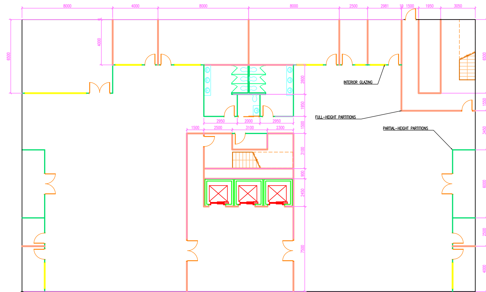
ROOM AND PARTITION LAYOUT FOR GROUND FLOOR (SCALE 1:200, UNITS IN MM)
