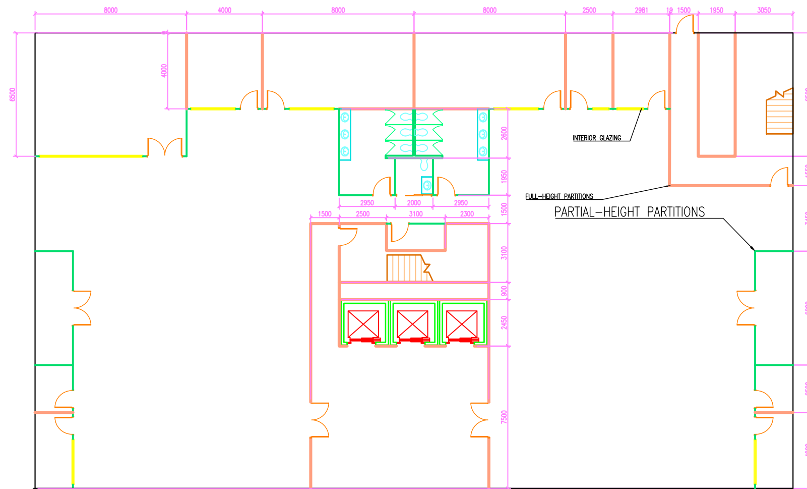
ROOM AND PARTITION LAYOUT GROUND FLOOR (SCALE 1:200, UNITS IN MM)
