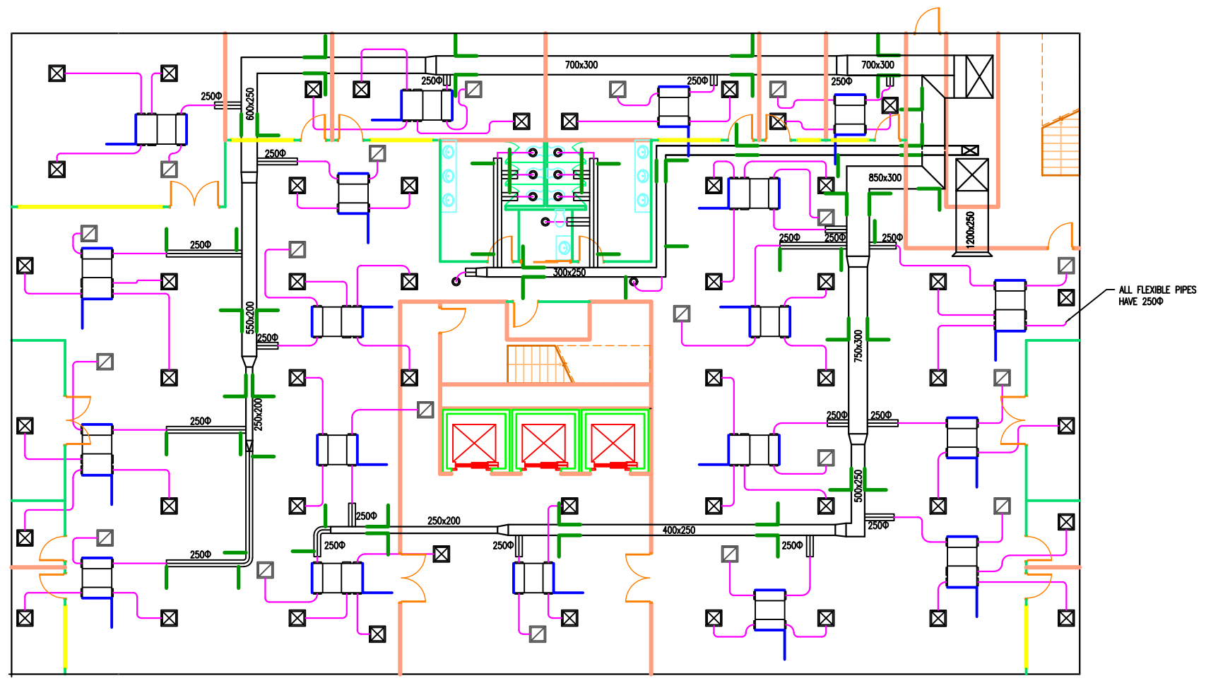
HVAC LAYOUT FOR GROUND FLOOR (SCALE 1:200, UNITS IN MM)
