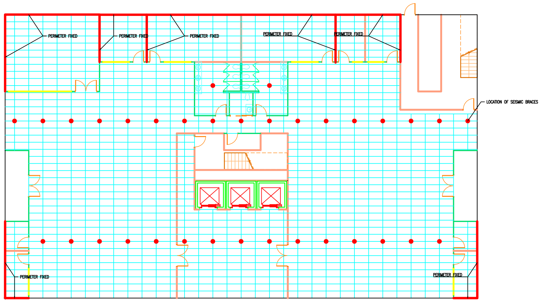
CEILING LAYOUT FOR GROUND FLOOR (SCALE 1:200, UNITS IN MM)
