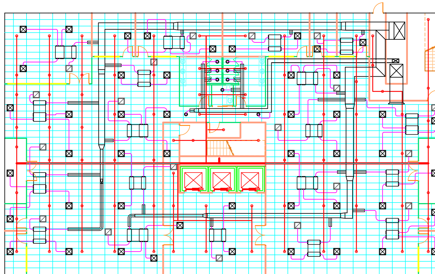
ABOVE CEILING LAYOUT FOR GROUND FLOOR (SCALE 1:200, UNITS IN MM)
