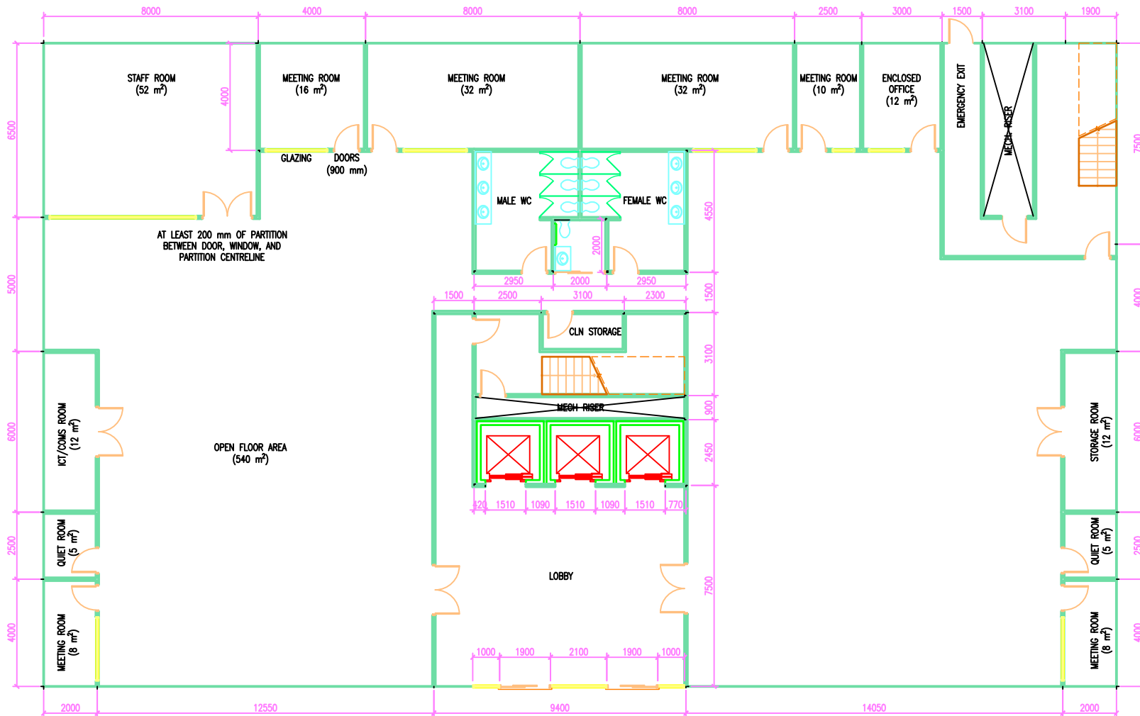
GROUND FLOOR LAYOUT (SCALE 1:200, UNITS IN MM)
